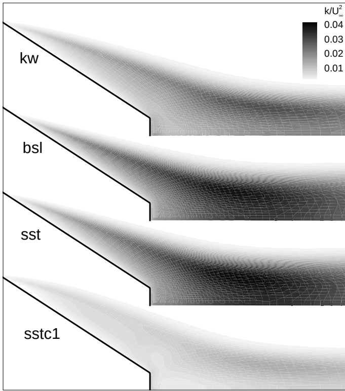
Figure 10. Contours of normalized turbulent kinetic energy as obtained using the different two-equation models.
