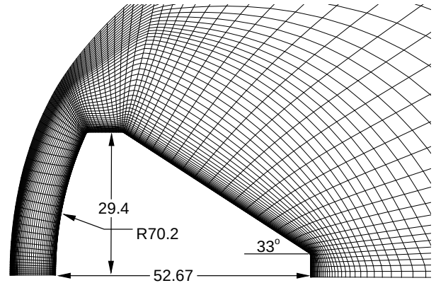
Figure 1. Computational Domain in the vicinity of the vehicle
