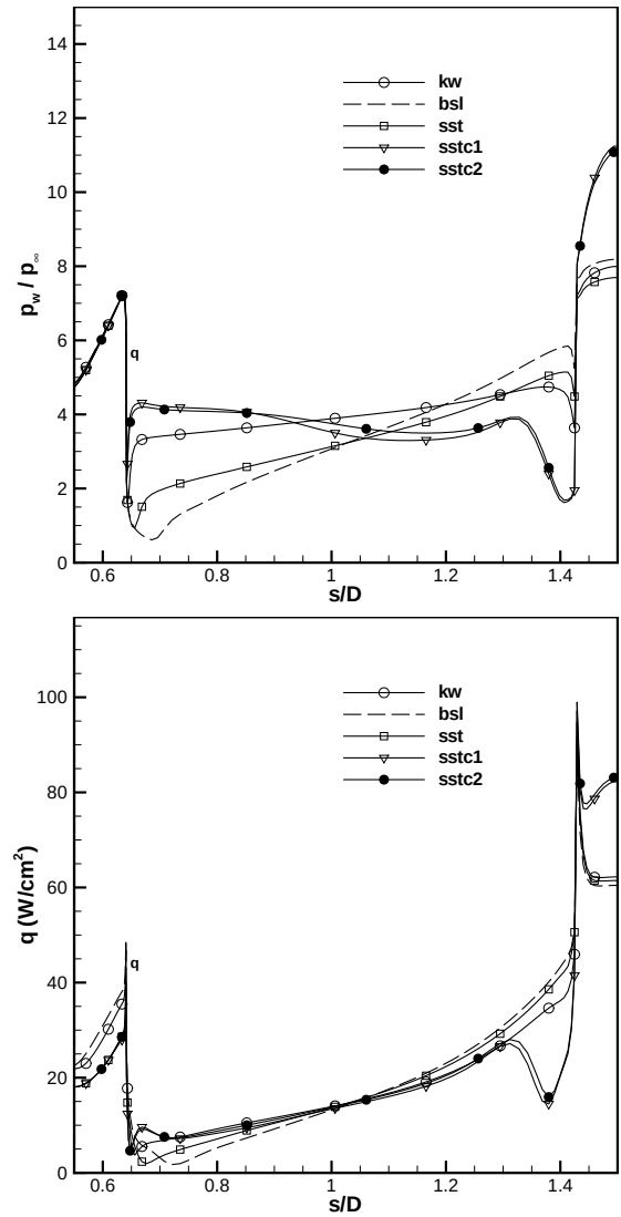
Figure 11. Comparison of afterbody normalized wall pressure and heat transfer rate predicted by the different two-equation model and their variants.
