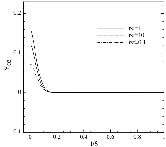
Fig. 13 Change in Y_{O_2} in the boundary layer at s/D = 0.52 (first expansion corner) due to variations in reaction rates.
