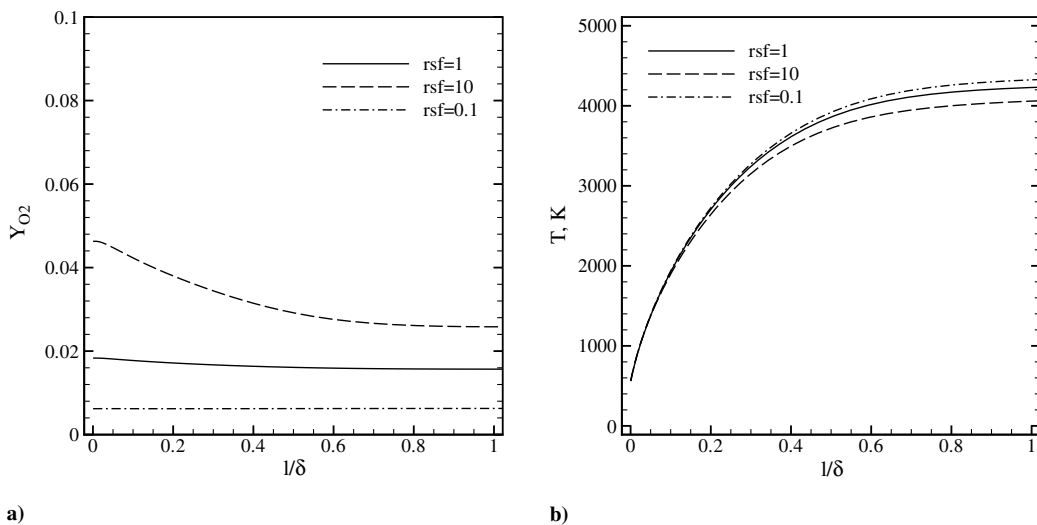
Fig. 15 Profiles of a) Y_{\text{O}_2} and b) temperature in the thermal boundary layer at the base stagnation point.
