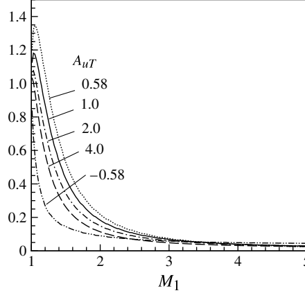
FIGURE 6. Ratio of downstream to upstream values of the correlations \overline{(\omega'_z \rho'_{,y}) / \omega_z'^2} (\bar{u} / \bar{\rho}) as computed using linear theory.
