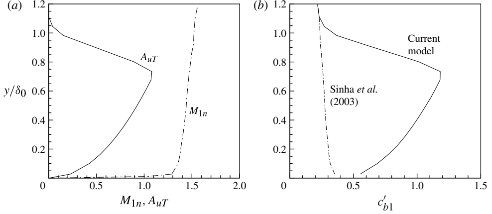
FIGURE 13. Variation of model parameters A_{uT} , M_{1n} and c'_{b1} in a 24° compression ramp SBLI flow. The wall-normal distance y is normalized by the undisturbed boundary layer thickness \delta_0 upstream of the interaction.
