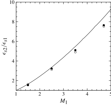
FIGURE 11. Comparison of \epsilon_s -amplification across the shock obtained from linear theory (line), DNS (●) and RANS computations using the current k - \epsilon model (○).
