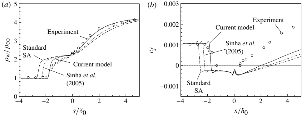
FIGURE 14. Comparison of (a) normalized surface pressure and (b) skin friction coefficient along a 24° compression corner obtained using different versions of the SA model with experimental data of Settles & Dodson (1994).
