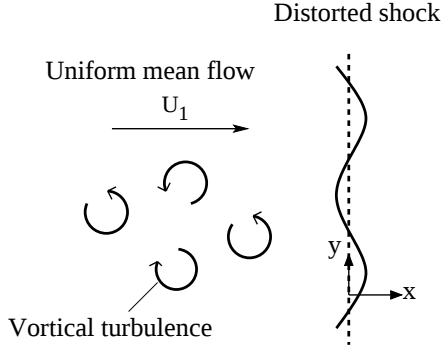
Figure 1. Schematic showing a shock wave distorted upon interaction with turbulent fluctuations.
