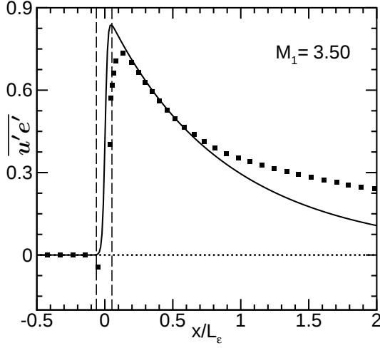
Figure 6. Variation of \overline{u'e'} along streamwise direction as per (9) (line) and DNS (symbol) for the case of M_1 = 3.50 . The vertical lines near x/L_\epsilon = 0 represent the mean shock thickness. Normalisation as described in figure 2.
