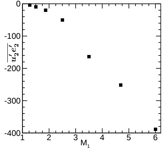
Figure 3. Peak \overline{u'_2 e'_2} values for varying upstream Mach numbers as predicted by conventional model with the shock-thickness taken from the DNS data. Note that the peak \overline{u'_2 e'_2} increases without bound as the shock-thickness is decreased, as it would be in an actual CFD simulation during grid-refinement. The results correspond to turbulent Mach number M_t = 0.15 just before the shock. Normalisation as described in figure 2.
