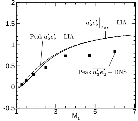
Figure 2. Variation of \overline{u'_2 e'_2} with upstream Mach number. The velocity fluctuation is normalized by the upstream mean velocity and the energy fluctuation is normalized by the downstream mean temperature and the specific gas constant R . All correlations are further normalized by the upstream TKE.
